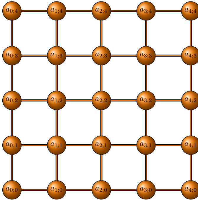
Figure 1.2: Depiction of a two-dimensional square lattice of interacting magnetic spins (Ising model [29]). Each spin is represented by a circular node. The interactions are represented by the lines between the nodes. These sorts of systems could give insight into condensed matter systems of interest, such as high-temperature superconductivity. The spins can be modelled by qubits. For highly entangled systems, exceeding approximately 30 qubits, classical computation becomes intractable [30].
