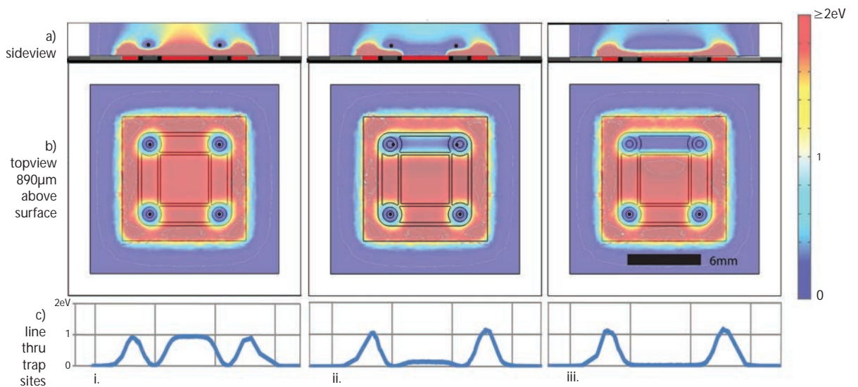
Figure 5.2: Series of simulations for trapping ^{40}\text{Ca}^+ ions in an addressable array of point ion traps with an inter-trap spacing of 6 mm. Top: a) series of simulations showing a slice through the pseudopotential field in eV through the middle of the two trapping sites which share an addressing electrode. Middle: b) series of simulations showing a slice through the pseudopotential 890 \mu\text{m} above the surface of the trap. Bottom: c) The pseudopotential along a line connecting the two trapping sites. From left to right (i-iii), the potential of the addressing electrode V_{\text{adj}} is ramped from 100% of V_{\text{nom}} (215 V 10 MHz) to 0 volts. Initially (i), the two ion traps are fully separated and form two well-isolated point quadrupole ion traps. In between (ii), V_{\text{adj}} is 43% of the nominal trap voltage and the trap frequency has been reduced. (iii) V_{\text{adj}} is at ground and the two addressed ion traps in the array are formed into a linear ion trap.
