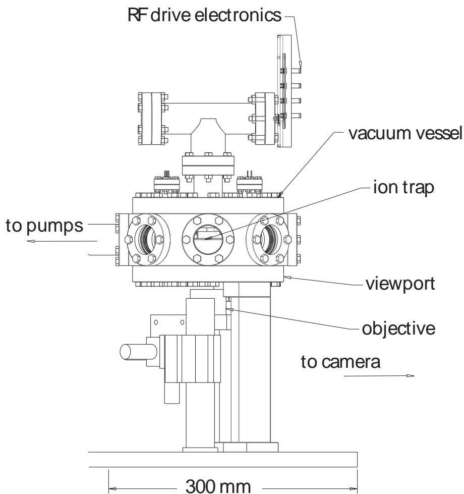
Figure 4.1: Above is a drawing of the vacuum setup for testing planar electrode ion traps. Lasers for cooling and photoionization have access through the viewports on the side of the vacuum vessel. Imaging of the ions is done through a viewport on the bottom of the vacuum vessel, through an objective. The vacuum pumps on the left include a Ti-sublimation pump and an ion getter pump. RF feedthroughs on the top allow for the trap to be driven by the RF electronics.
