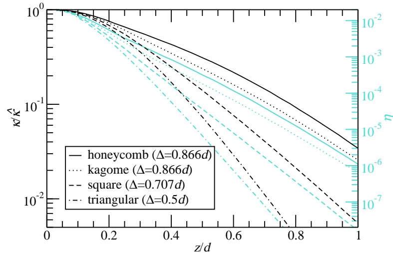
Figure 3.10: Normalized trap curvature and depth for various geometries of 2D trap arrays as given by Schmied [163]. The bottom axis shows the ratio of the ion height z to the inter-trap spacing d . The curves show the performance of various topologies of 2D lattices of ion traps, where the performance is given by the trapping depth efficiency \eta and the ratio \kappa/\hat{\kappa} of the electric field's curvature \kappa to the curvature of an optimized surface ring-trap \hat{\kappa} [160]. The efficiencies and curvatures drop-off exponentially with increasing z/d ratio. Reprinted figure with permission from R. Schmied, Phys. Rev. Lett. 102, 233002 (2009). Copyright 2009 by the American Physical Society.
