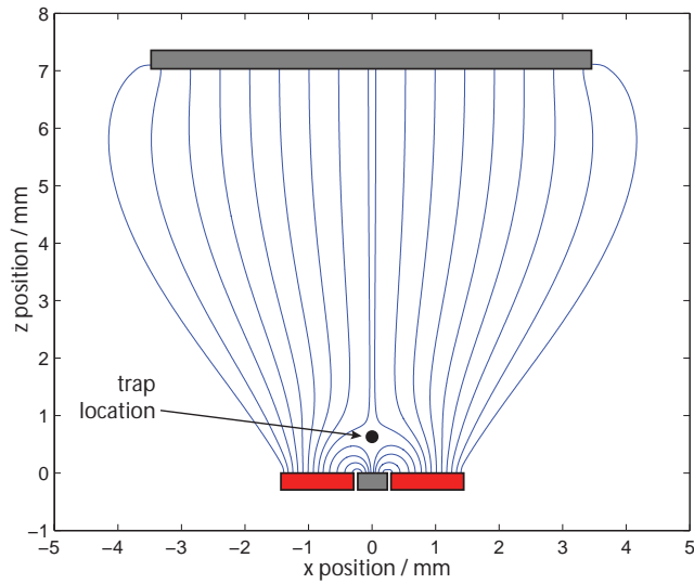
Figure 2.3: The 2D simulation results of a planar electrode quadrupole ion trap. Four electrodes, two with a positive voltage, and two with a negative voltage, create a quadrupole near the ion's trapping site. One of the negative electrodes is 7 mm above the trap surface created by the rest of the electrodes. The ions are trapped about 0.5 mm above the surface of this trap.
