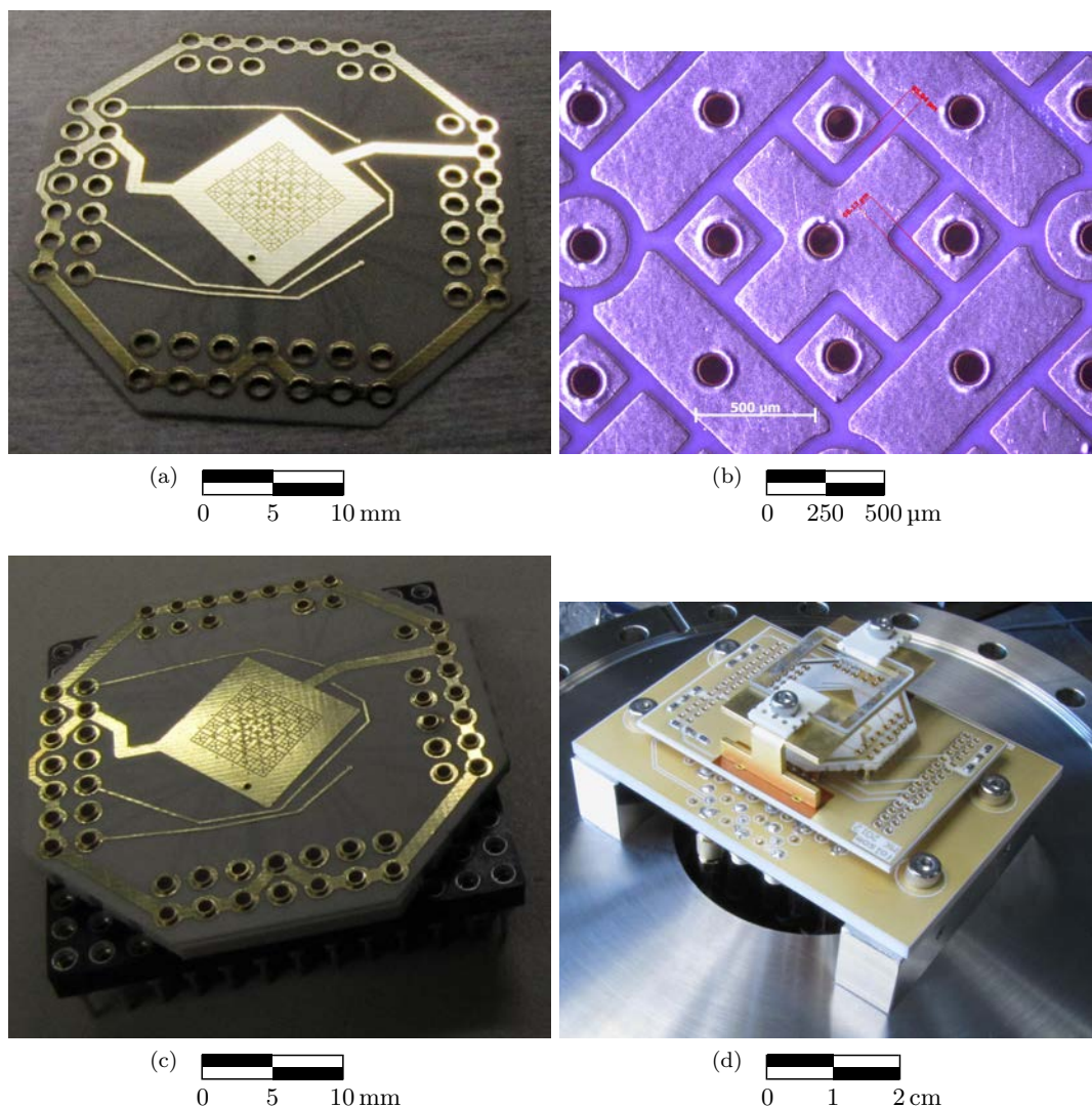
Figure 6.5: Fabrication of the Folsom ion trap. (a) printed circuit board. (b) detail of the center electrodes' structure after plating with gold. (c) connectorized trap. (d) trap plugged into the vacuum filter board and connector board. A transparent ground plane is mounted 7 mm from the trap surface. The entire assembly is then installed in the vacuum chamber with the trap facing downwards.
