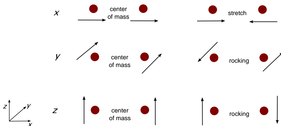
Figure 2.7: The motional modes of two ions in an ion trap. There are 6 motional modes to consider.
