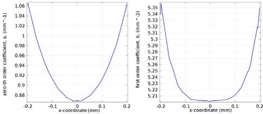
Figure 3.8: Results of a finite element method (FEM) simulation of the electric field inside a trap with geometry described by figure 3.7 given in terms of the zeroth order electric-field coefficient a_x (a) and first order electric-field coefficients b_x (b). Because (b) is the derivative of the electric field, which is a derivative of the simulated potential, the granularity of the FEM meshing results in some jaggedness of the coefficients a_x and b_x .
