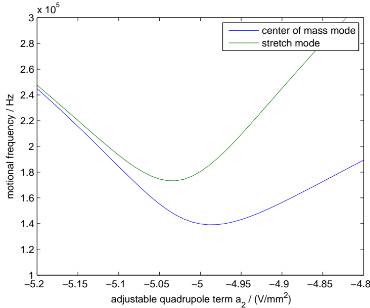
Figure 3.3: The motional frequencies during the merging of a double-well formed from an adjustable quadratic term a_2 and an overall quartic term.
