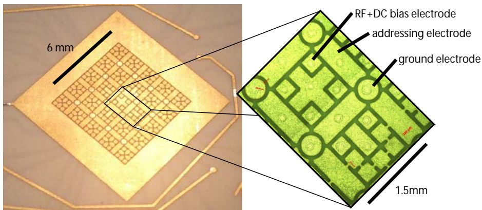
Figure 6.1: Fabricated trap. Inside the diamond area, is a 4 \times 4 array of planar point quadrupole ion traps. A microscope close-up of the middle 2 \times 2 section of the trap shows details of the electrode structure. The nominal trapping sites (circular electrodes \varnothing 400 \mu\text{m} ) are 1.5 mm from each other.
