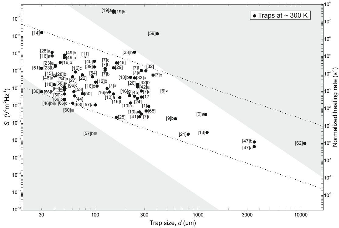
Figure D.1: Spectral density of electric-field noise S_E as a function of the distance d from the ion to the nearest electrode, for traps operated nominally at room temperature. Data points are taken from the relevant references in table D.1. On the right, the ordinate scale is given as the equivalent heating rate of a ^{40}\text{Ca}^+ ion with a motional frequency of \omega_x = 2\pi \times 1\text{ MHz} . The shaded regions indicate an envelope scaling with d^{-4} . The dotted lines indicate an envelope scaling with d^{-2} . See reference [125] for discussion, including the uses and significant limitations of plotting such data on a single graph.
