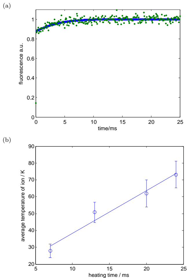
Figure 6.18: Heating-rate measurements using the recooling method. (a) fluorescence rate as a function of time during recooling (point data) and the recooling-model fit (solid line), after allowing the ion to heat for 24 ms. (b) the average energy of the ion, given by the recooling model, as a function of the heating time. A least-squares fit (dotted line) gives a heating rate of approximately 2.5 K/ms
