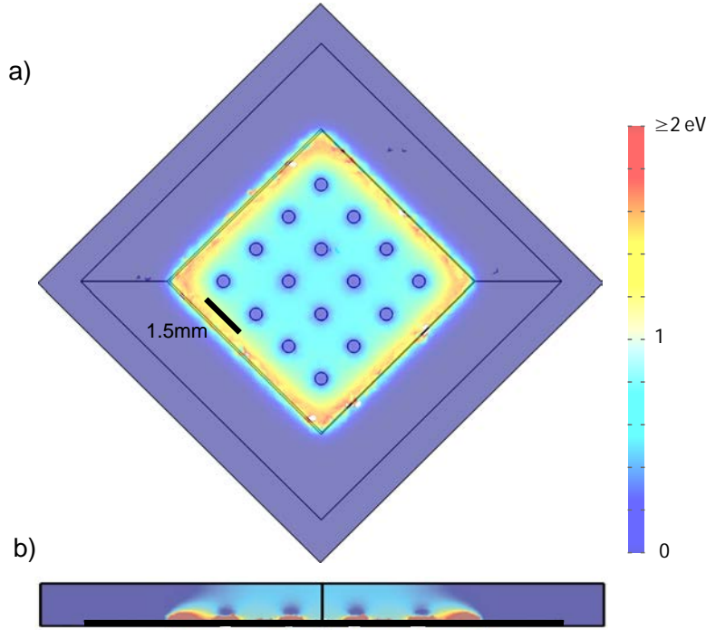
Figure 6.3: Simulation of Folsom trapping ^{40}\text{Ca}^+ ions showing the pseudopotential (eV) 375 \mu\text{m} above the surface of the trap (above) and also from the side diagonally through the trap. A ground plane sits 1.5 mm above the surface of the trap. The trapping depth is about 0.5 eV. All RF electrodes are fully driven with a voltage amplitude of 125 V and a frequency of 10 MHz.
