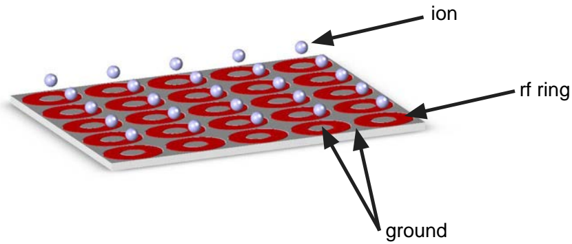
Figure 3.1: A representation of how a 2-dimensional 5 \times 5 array of planar point ion traps might appear. Each ring has a radio-frequency voltage applied to it. Inside each ring is a circular ground electrode. Outside the ring a ground potential can be applied or a distant ground such as the vacuum chamber can be used. The ions are trapped above the circular ground electrodes.
