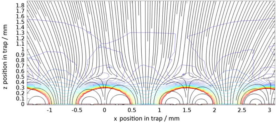
Figure 6.4: A cross section of the trapping fields in the trapping array Folsom. The field lines are shown in black and the pseudopotential is shown as color coded contours (same scale as in figure 6.3). Because of the 3D nature of the electric-field simulation, the field lines disappear into and out of the cross-section plane. The RF and DC ground electrodes are seen on the bottom of the figure.
