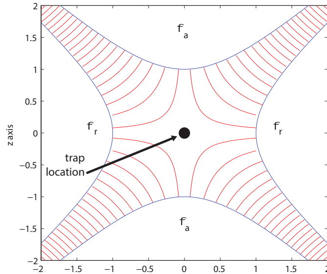
Figure 2.2: Geometry of hyperbolic electrodes. Equipotential lines satisfying the relation \phi = \alpha_t(r^2 - z^2)/2 form a hyperboloid of revolution around the z -axis. \phi_a is the axial electrode voltage and \phi_r is the radial electrode voltage. Both sets of electrodes here are drawn without units a distance d = 1 from the center of the trap. Actual dimensions and voltages would define the field gradient \alpha_t . Red lines show the quadrupole field lines, which meet the trap electrodes normal to the surface. At the center of the trap, the electric field is zero and is where ions could be trapped. Equipotential surfaces with the applied voltages can be made of metal and provide the trapping field for an RF Paul trap.
