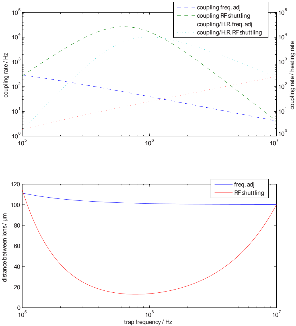
Figure 3.11: A comparison of addressing the interaction of two nearest neighbors in a 2D array, by either RF displacement or shared frequency tuning. The top figure shows both the coherent coupling rate of motion between the ion in each trap (dashed lines) and the normalized coupling rate vs. the heating rate (dotted lines), as a function of the trap frequency during addressing. The heating rate is assumed to be inversely proportional to the trap frequency \omega_x squared, as it would be from a source of electric-field noise (see eq. 2.92) with a 1/f profile. One can see that, a trap with, where the nearest neighbors are addressed with RF displacement (upper dashed line) allows the coupling to be increased almost three orders of magnitude more than just with shared frequency tuning (lower dashed line). Furthermore, the RF displacement allows the normalized coupling rate vs. heating rate to be increased during the RF displacement (upper dotted line) vs. the shared frequency addressing (lower dotted line).
