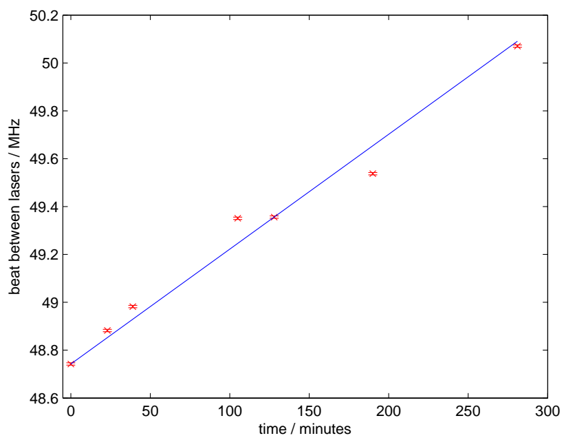
Figure 4.2: Drift rate of 729 nm laser locked to the optical cavity. The laser drifts at a rate of about 80 Hz/sec when locked to the cavity.
