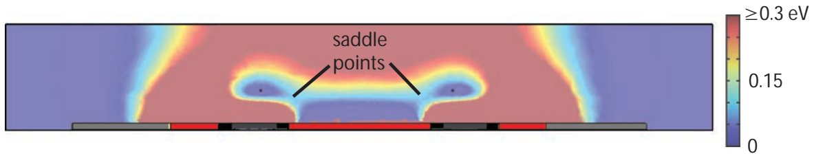
Figure 5.3: A closer look at the simulation results (from figure 5.2.a.ii.) when V_{\text{adj}} is at 43% of V_{\text{nom}} . Here the color scale has been set so that the saddle points are easier to see. A trap appears over the addressing electrode. The trapping locations are indicated by dark points in the spherical trapping potentials. The ion-ion distance has been also reduced by 10% compared to the distance with full voltage on the addressing electrode. The potential of the saddle point (here \sim 0.1 eV) between the new trap over the addressing electrode and the point quadrupole ion traps falls with the square of the addressing electrode’s voltage. However at all times the ions are trapped within the array by a strong potential.
