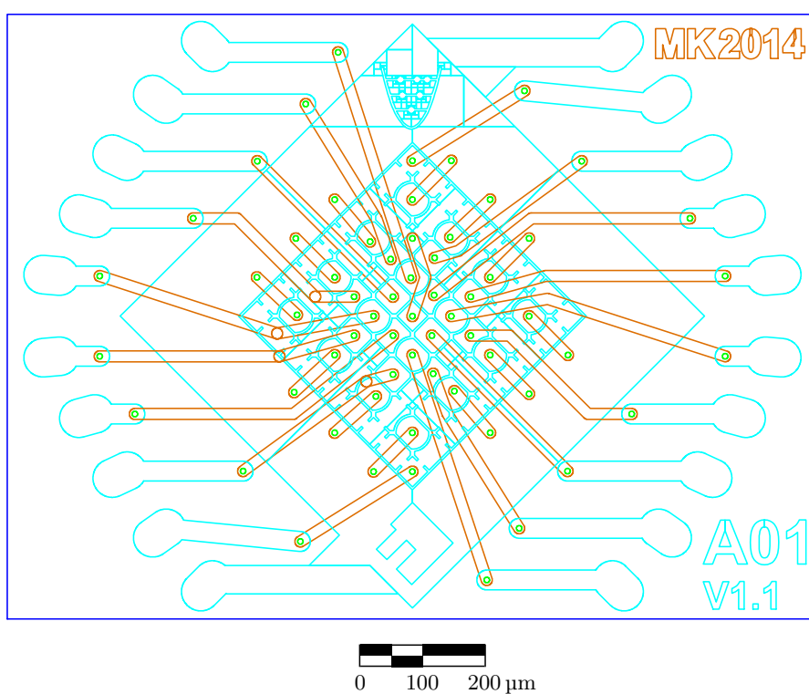
Figure C.7: Ziegelstadl trap array v1.1, all layers.
