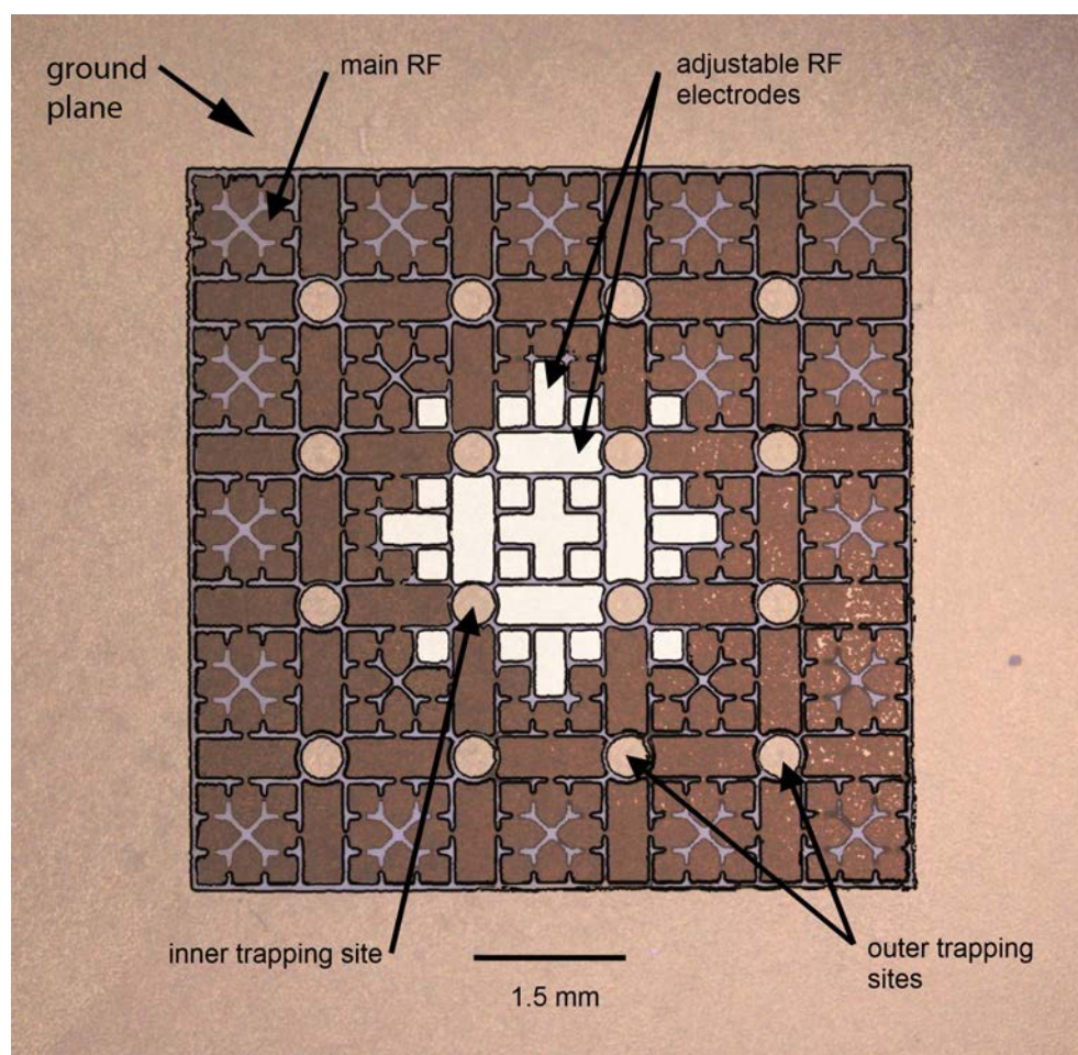
Figure 6.2: False color image of fabricated trap layout. The nominal trapping sites (circular electrodes \varnothing 400\ \mu\text{m} ) are 1.5 mm from each other. The main RF is colored darker than the adjustable RF electrodes (bright). DC electrodes are colored light brown. The inner 2 \times 2 trapping sites have many individually adjustable electrodes so that micromotion can be minimized.
