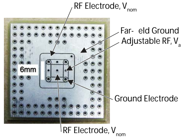
Figure 5.1: Geometry of the electrodes used for the simulation of trapping ^{40}\text{Ca}^+ ions in a 2 \times 2 array of addressable ion traps as well as for the trapping of charged dust particles. Above each circular ground electrode is a point quadrupole ion trap. The trap is implemented on a circuit board and has the same physical layout as an industry-standard PGA101 integrated-circuit chip carrier so that it can be plugged into a standard socket.
