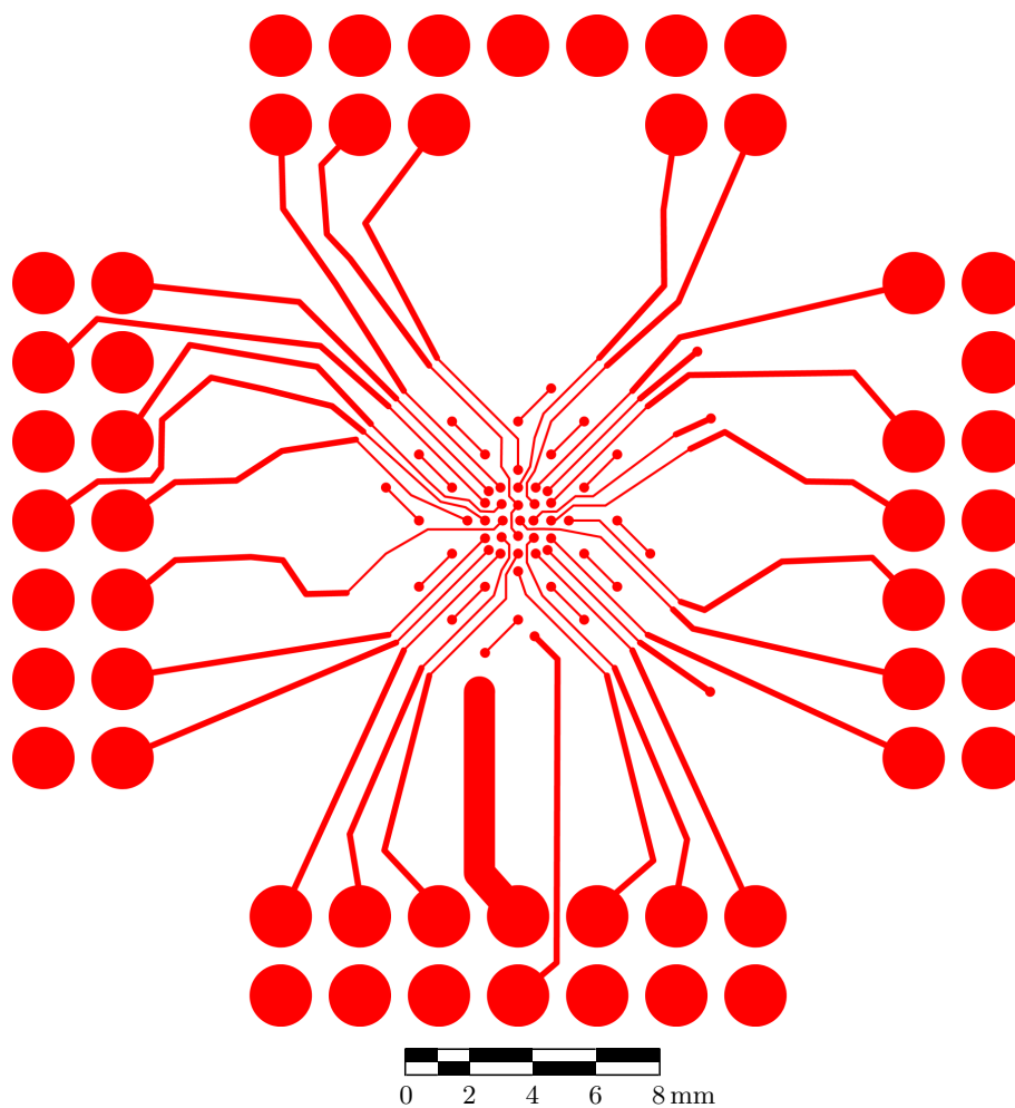
Figure C.5: Folsom trap array, bottom layer.
