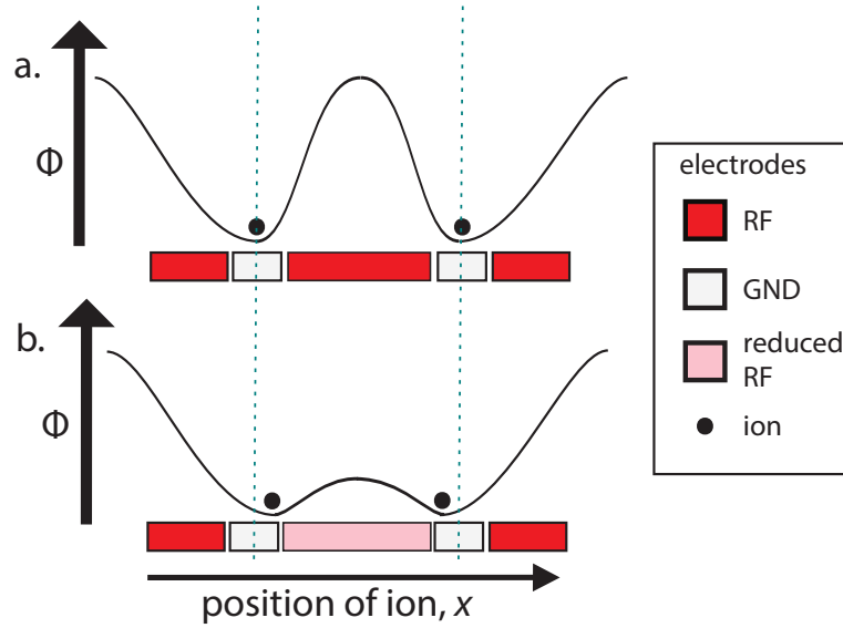
Figure 3.4: A double-well pseudopotential along a line connecting two neighboring ions, each in a point ion trap with a shared adjustable RF electrode. There are three types of electrodes in this configuration. The first are ground electrodes, which have no RF voltage applied. The second are the main RF electrodes, which have a fixed amplitude RF voltage applied to them. The third kind of electrode is an adjustable RF electrode. Figure 3.4a depicts the double-well pseudopotential \phi of an array when all RF electrodes have the same amplitude. And figure 3.4b shows the pseudopotential \phi when an adjustable RF electrode, in between the two trapping sites, has its RF voltage amplitude reduced. When the adjustable voltage amplitude is decreased, the electric field between the two trapping sites decreases as described below. The pseudopotential then decreases as the electric field squared (see eq. 2.25).
