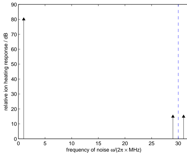
Figure E.1: The relative efficacy of heating, in dB, with a motional frequency \omega_x of 2\pi \times 1 MHz and a trap drive frequency \Omega_{\text{rf}} of 2\pi \times 30 MHz in the presence of a spectral noise S_E which is constant over the frequencies of interest. The efficacy of the heating due to noise at the motional sidebands (29 and 31 MHz) is reduced by about 65 dB or a factor of 1800 compared to the heating from noise at the motional frequency (1 MHz).
