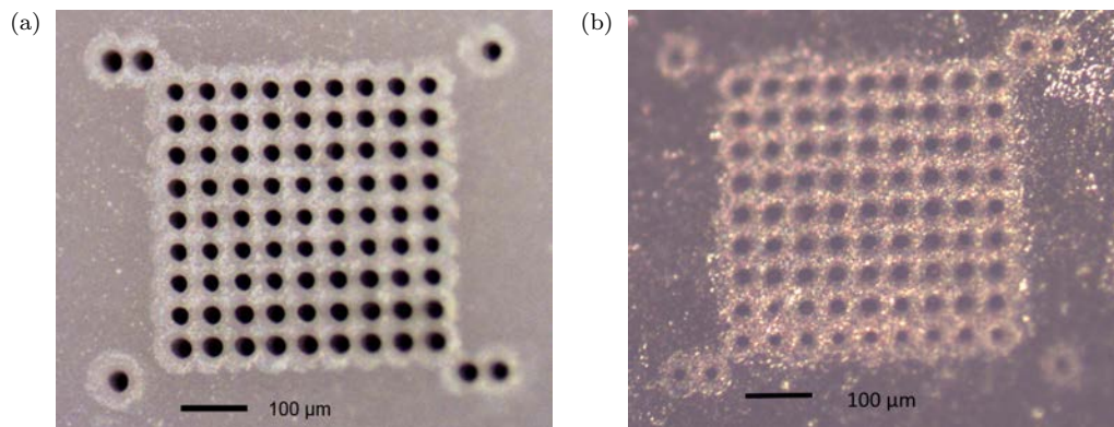
Figure 7.4: Steps showing Matrix fabrication, 2nd attempt. A laser drilled alumina substrate (a) before metalization (b) after gold metalization using an electro-less gold plating process.
