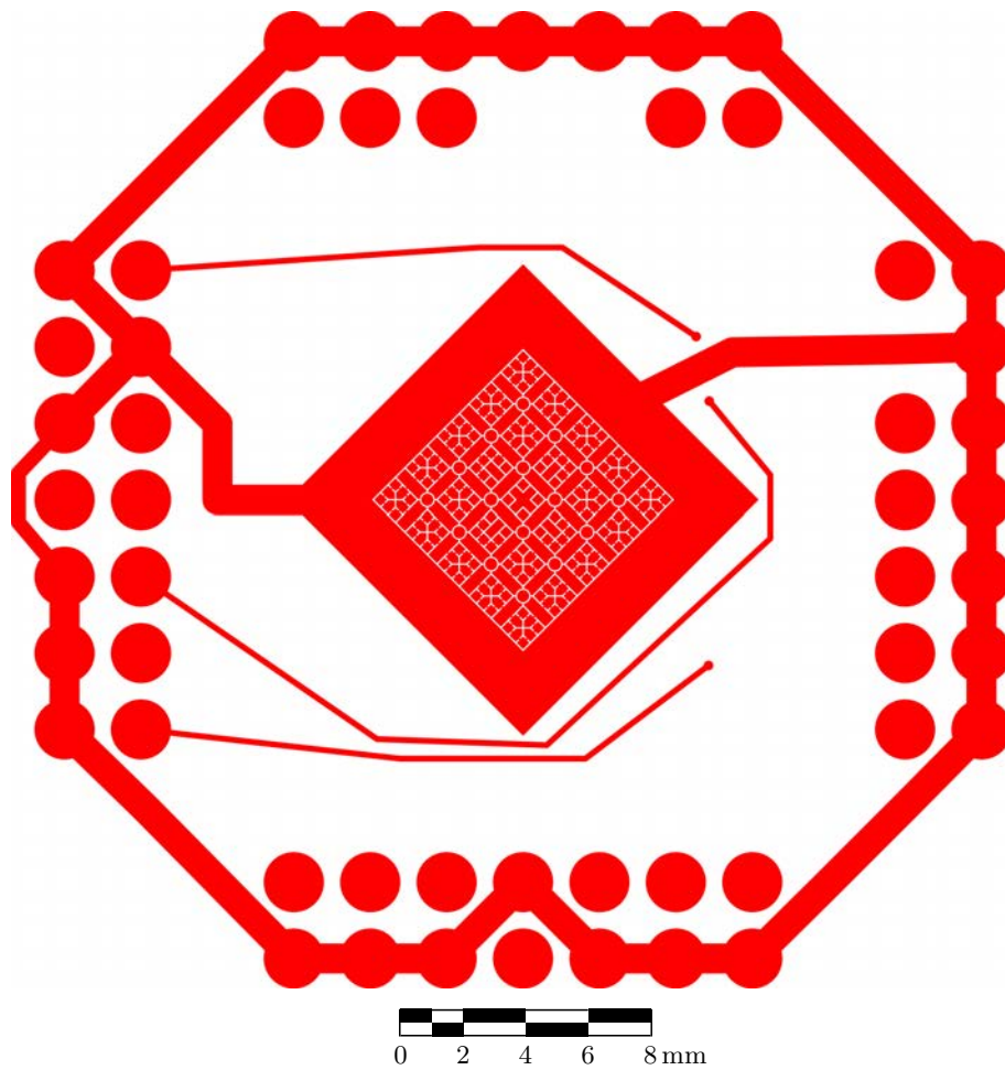
Figure C.4: Folsom trap array, top layer.
