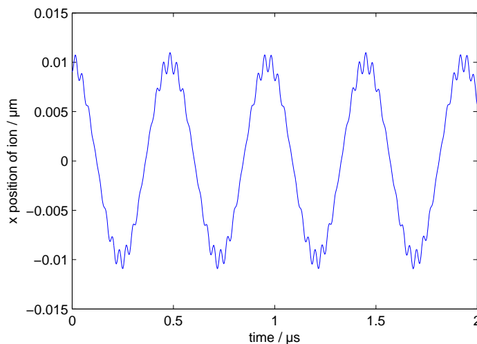
Figure 2.14: An example of the classical motion of an ion in a quadrupole ion trap. The slow oscillations are at the secular frequency of 2 MHz with an amplitude of 10 nm. The fast oscillations are at the trap drive frequency of 30 MHz. The trapping parameter q_x is approximately 0.19, which sets the amplitude of the micromotion relative to the secular motion.
