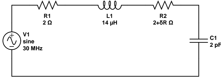
Figure E.3: The schematic used for estimating the flicker noise in the thin film electrode. The trap is driven with a resonant circuit (where the resonator’s inductance cancels the trap’s capacitance), so that variations in the trap electrode’s resistance \delta R cause a corresponding change in the RMS current flowing in the circuit. Here, the resistance of the thin-film metal electrode is assumed to be the predominant loss in the system, so that the RF resonator and signal source are matched to drive this 2\ \Omega load. This means that at steady state, when \omega_x \ll \Omega_{\text{rf}} , the RMS trap drive current variation due to a change in the resistance of the thin-film electrode is 1/2 the change of the resistance; i.e. a 2% change in resistance from flicker noise, would result in a 1% change in the RMS current.
