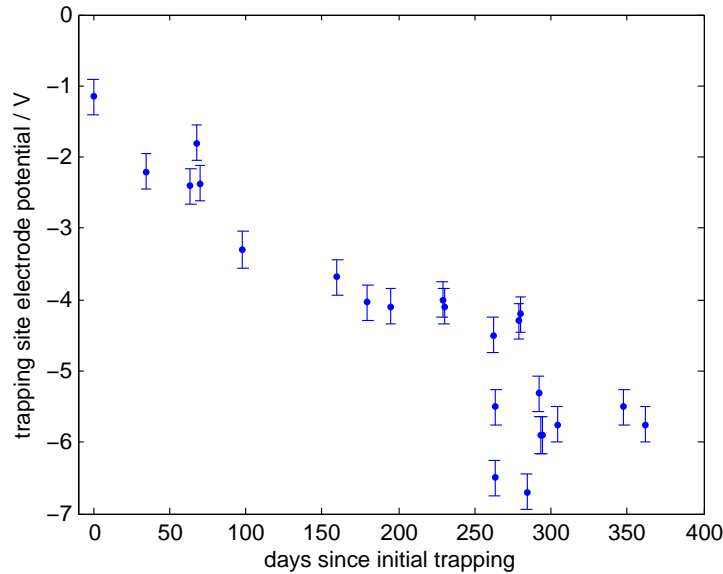
Figure 6.15: Above is the required voltage applied to the circular trapping-site electrode so that trapping was possible. Over a year of experimentation, the required voltage went from approximately -1 V to -6 V.
