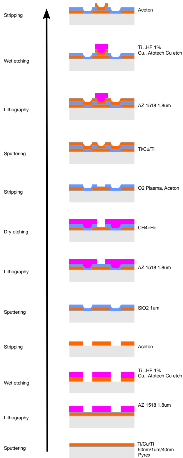
Figure F.1: Fabrication steps (ordered from bottom to top) for Ziegelstadl v1.0 Cu electrodes.
