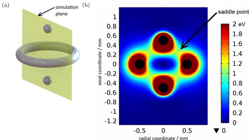
Figure 2.4: The geometry of a ring trap (a) and the simulation of the pseudopotential field in the simulation plane (b). The saddle points in the pseudopotential field give the trapping depth the ion experiences. The electrodes are about 1 mm apart on-center and 200 \mu\text{m} in diameter. An RF potential of amplitude 100 V and 30 MHz is applied between the ring and electrode. The resulting pseudopotential is plotted in eV.
