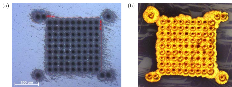
Figure 7.3: Steps showing Matrix fabrication. A laser drilled alumina substrate (a) is metalized with gold electro-plating so that vias form connections through the substrate (b).
