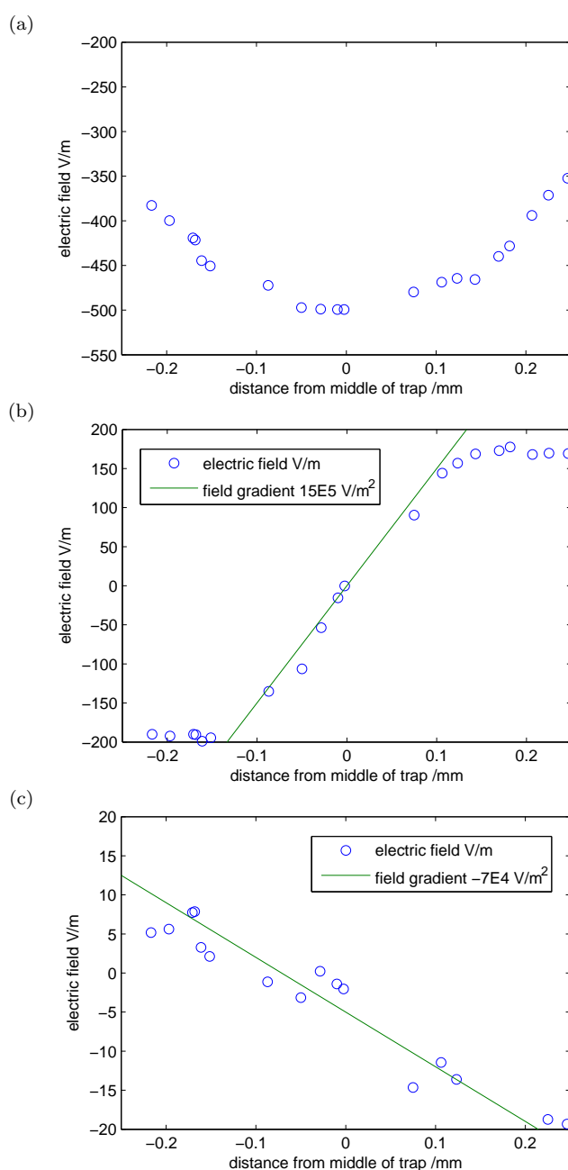
Figure 6.7: The electric fields as a function of the x position around the center of a trapping site for the various applied voltage configurations. A procedure analogous to that given in section 3.5.2 is used, so that the simulations are run as follows: For the dipole-like electrode configuration figure (a), corresponding to coefficient a , the two near RF electrodes have a voltage of +1 \text{ V} and -1 \text{ V} while the rest of the array is at ground. For the quadrupole-like configuration figure (b), corresponding to coefficient b , the two nearby electrodes have a voltage of +1 \text{ V} , while the nearby ground electrode and ground plane are set at 0 \text{ V} . For the residual array RF figure (c), term c , all the RF electrodes, except for those neighboring the trapping site are set to +1 \text{ V} , while all other electrodes, including the neighboring RF electrodes, are set at -1/2 \text{ V} . In order to compute the quadrupole coefficients, a line has been fitted to the simulation data, so that the gradient of the electric field can be seen. The extra field has the effect of producing a quadrupole like field which is only about 5% compared to the adjustable RF electrode’s quadrupole term. For these simulations, a ground plane sits 7 mm above the surface of the trap.
