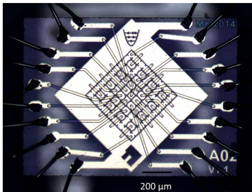
Figure 7.1: Above is a microscope image of a miniaturized 2D array of ion traps, called Ziegelstadl currently being tested. Here it is shown mounted and wire bonded to a filter board.
