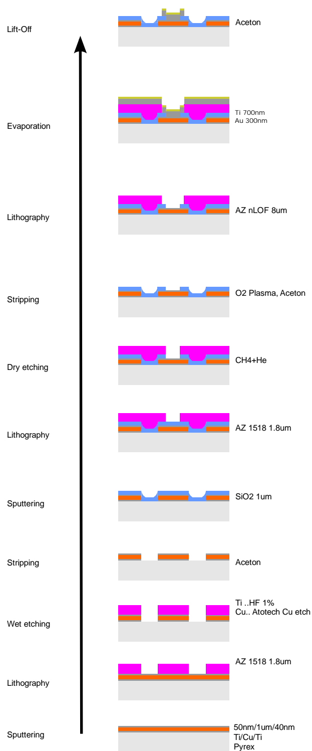
Figure F.2: Fabrication steps (ordered from bottom to top) for Ziegelstadl v1.0 Au/Ti electrodes.
