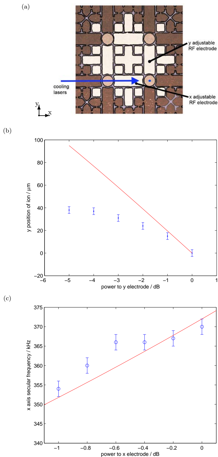
Figure 6.16: Results of adjusting the power to the adjustable electrodes. (a) the configuration of the laser-cooling and electrode adjustment. (b) the ion position versus the applied RF power. (c) the frequency of the ion trap versus the applied RF power. Also shown are the models of RF displacement and frequency tuning with a single parameter fit.
