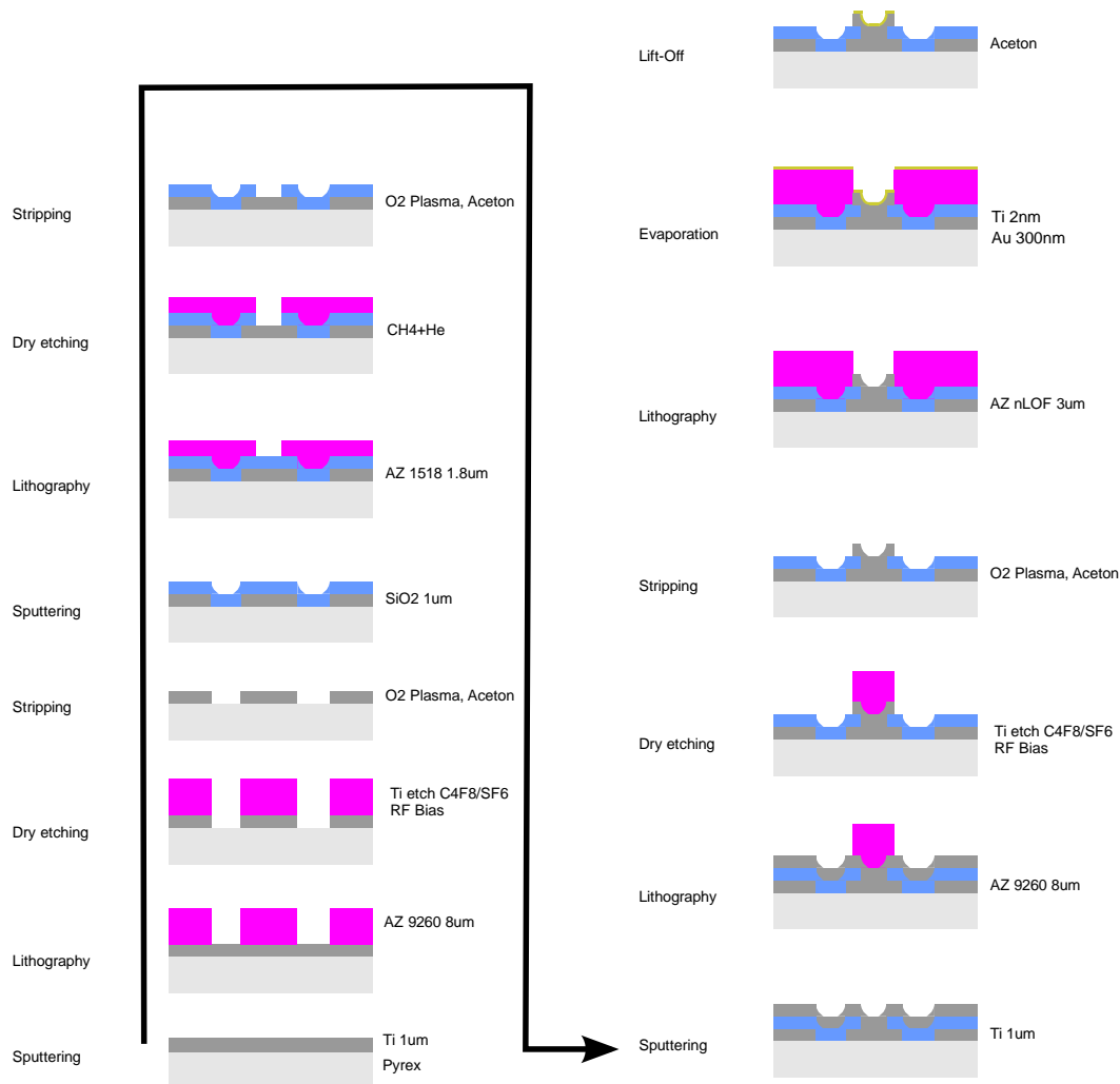
Figure F.3: Fabrication steps (ordered from bottom to top and left to right) for Ziegelstadl v1.1 Wafer #1.
