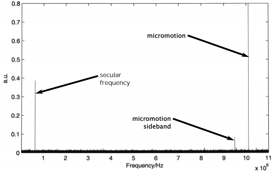
Figure 6.17: The secular and micromotion peaks in the power spectral density of the time arrivals of the fluorescence photons. Most prominently in the figure, is the micromotion peak at the trap drive frequency of 10.1 MHz. The secular frequency peak can also be seen. For the conditions shown, the secular frequency \omega_x was approximately 600 \times 2\pi kHz. Also visible is the micromotion sideband at approximately 10.1 - 0.6 = 9.5 MHz. The appearance of the micromotion sideband is due to the excited secular motion of the ion mixing with the micromotion
