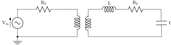
Figure 6.8: Schematic representation of a tank resonator, which uses a perfect transformer to match the resonator’s resistance R_L on resonance to that of the source impedance R_S of the voltage source V_{in} .
