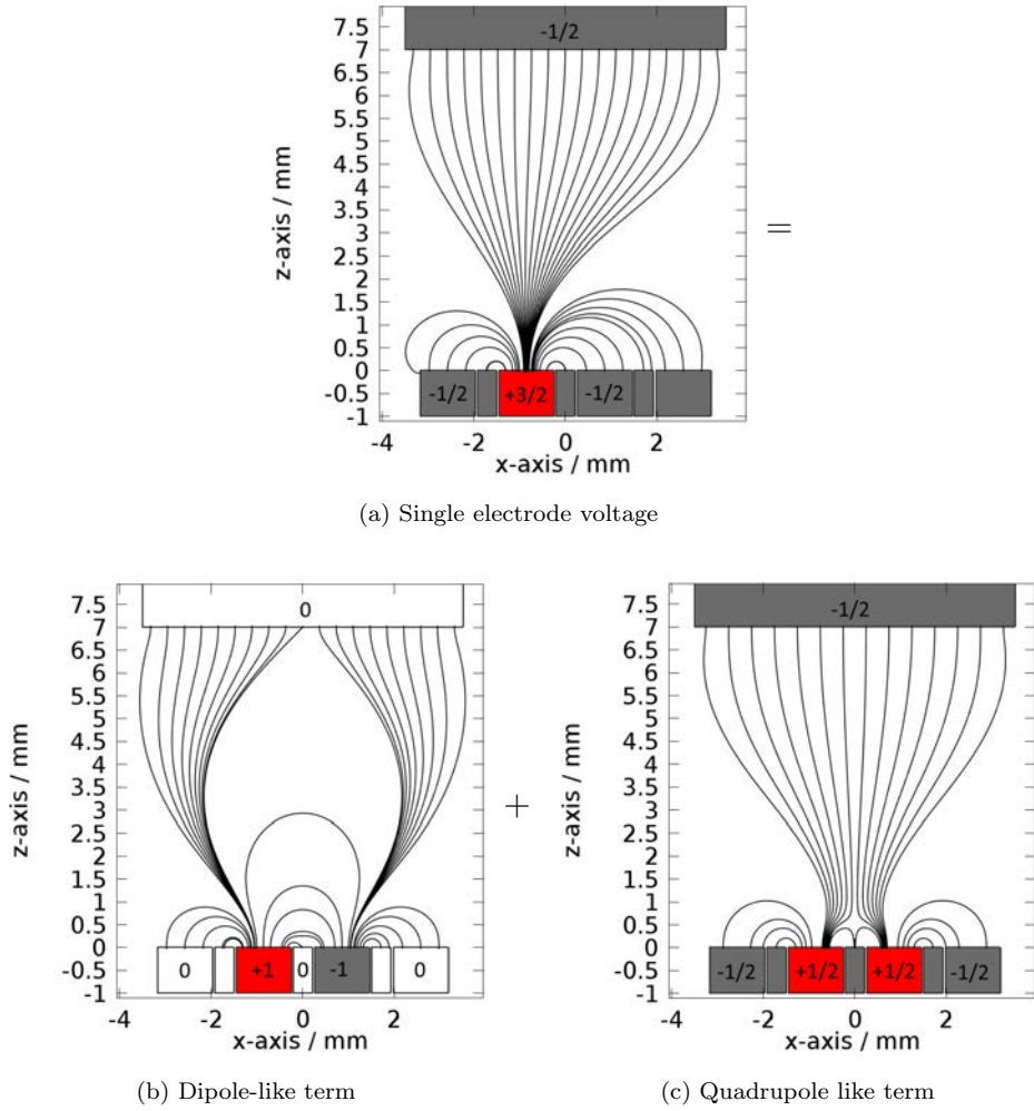
Figure 3.9: The decomposition of the field due to a single voltage in a 2D array of ion traps (a) into a dipole like field (b) and a quadrupole like field (c).
