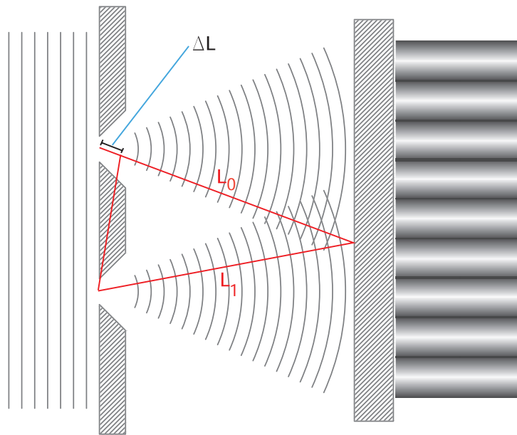
Figure 1.1: Quantum interference is much like classical wave interference, except that each individual quantum (or particle) has a probability amplitude wave associated with it. Above is a figure showing how a travelling particle (say a photon or electron) can interfere with itself by going through two slits. The particle is in a superposition of states, where the particles goes through both the top and bottom slit. The interference pattern can be seen as the probability that the particle will be observed on the screen on the right.
