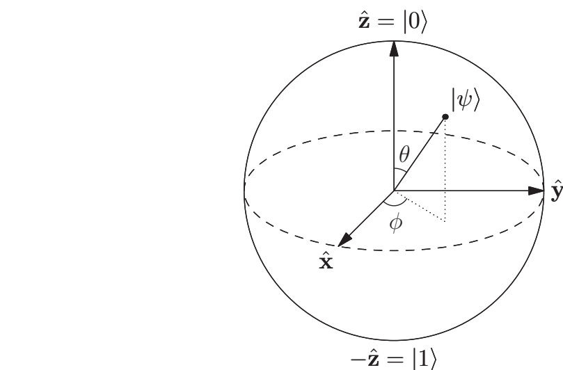
Figure 2.12: Bloch sphere representation of a qubit showing the relation between the angles \theta and \phi to a vector on the unit sphere, which represents the qubit |\psi\rangle .
