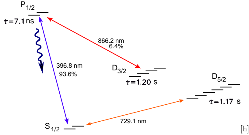
Figure 2.13: State detection using the electron shelving technique for ^{40}\text{Ca}^+ . Absorption of a single 729 nm photon causes an ion in the ground state to be excited to the D_{5/2} state. If the ion is in the D_{5/2} state, it will then cease to fluoresce in the presence of 397 nm radiation. If the qubit is encoded into the S_{1/2} and the D_{5/2} states, then this method can measure the qubit with more than 99.99% accuracy [114]
