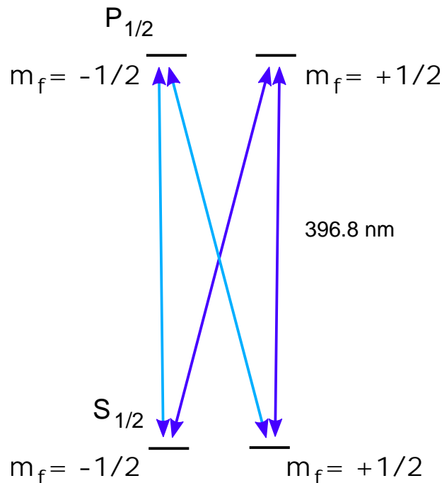
Figure 2.10: An illustration of dark states involving just the S_{1/2} and P_{1/2} Zeeman sublevels. Laser light can coherently excite the populations in each of the ground states to the two excited states. If the phase of the ground states is opposite, |-\rangle = (|m_F = -1/2\rangle - |m_F = +1/2\rangle)/\sqrt{2} , then they destructively interfere and the excited state population (and hence fluorescence) is reduced.
