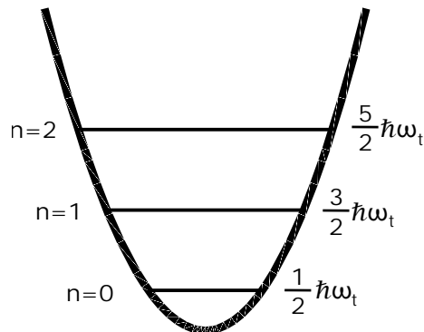
Figure 2.6: The Fock states (left) and the corresponding energy levels of the quantum harmonic oscillator. The energy levels are equally spaced and quantized. The lowest energy level has a non-zero amount of energy.
