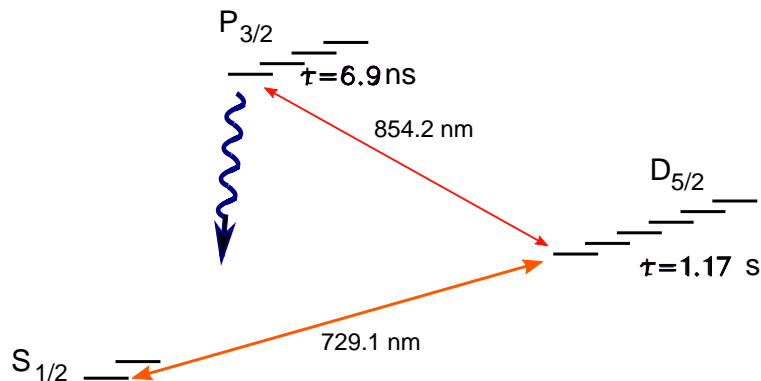
Figure 2.11: Sidband cooling of a ^{40}\text{Ca}^+ ion. After Doppler cooling and electronic state preparation to the S_{1/2}, m_F = -1/2 state, the application of a frequency selective RSB pulse can transfer the ion's state from S_{1/2}, m_F = -1/2 to D_{5/2}, m_F = -5/2 . Application of the 854 nm laser can then transfer the D-state population to P_{3/2}, m_F = -3/2 since this is the only dipole-allowed transition. The excited P_{3/2}, m_F = -3/2 then can only decay to the S_{1/2}, m_F = -1/2 state. If the Lamb-Dicke parameter \eta is small, then the 854 nm transition to P_{3/2} and the spontaneous decay to the ground state are both unlikely to increase the motional quantum number, and each cycle of this process should decrease the average phonon number by 1. Such a process can produce an ion in the motional ground state with more than 99.9% probability [100].
