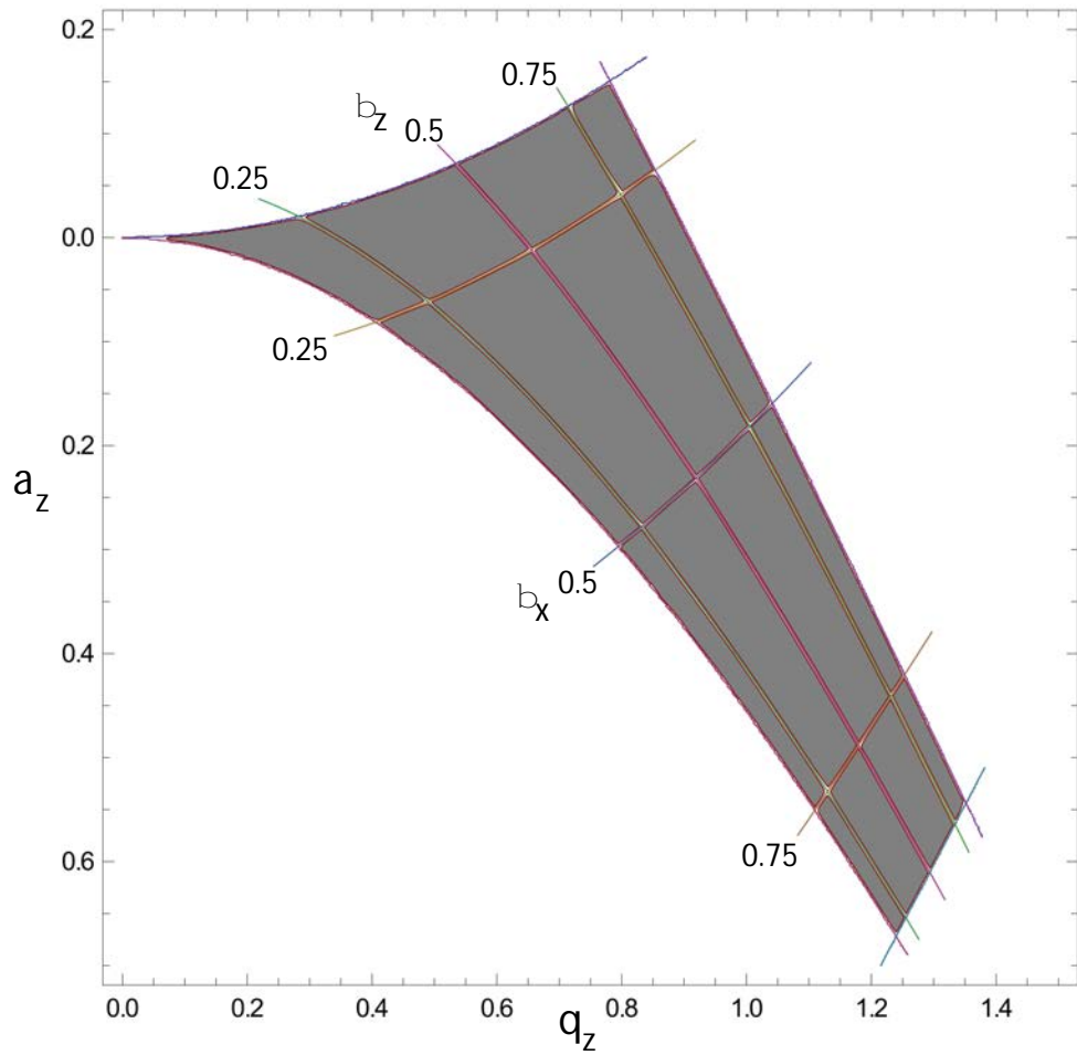
Figure 2.1: First stability region of the Mathieu equations for a spherical ion trap with respect to the trapping parameters q_z and a_z . Inside the shaded area, the Mathieu equations have a stable solution. There are an infinite number of much smaller stability regions, but most spherical ion trap experiments are performed inside this shaded region. For trap parameters outside a stable region, the ion's motion grows without bounds.
