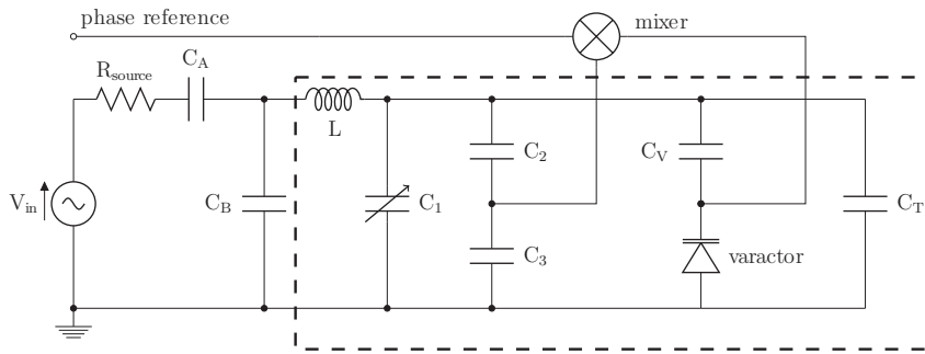
Figure 6.11: A schematic of the phase-locked RF resonator. A tank resonator is formed by the high Q inductor L and the capacitors to the right of it. The mixer locks the output phase of the resonator via the varactor diode.
