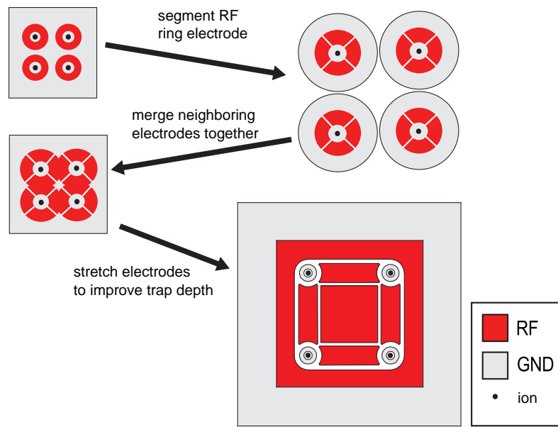
Figure 3.6: A representation of the conceptual process in going from a static 2-dimensional array of ion traps to an array where the neighboring ion-ion interaction can be addressed via the shared addressing RF electrode. Ions are trapped over each circular ground electrode when all RF electrodes are driven with equal voltage.
