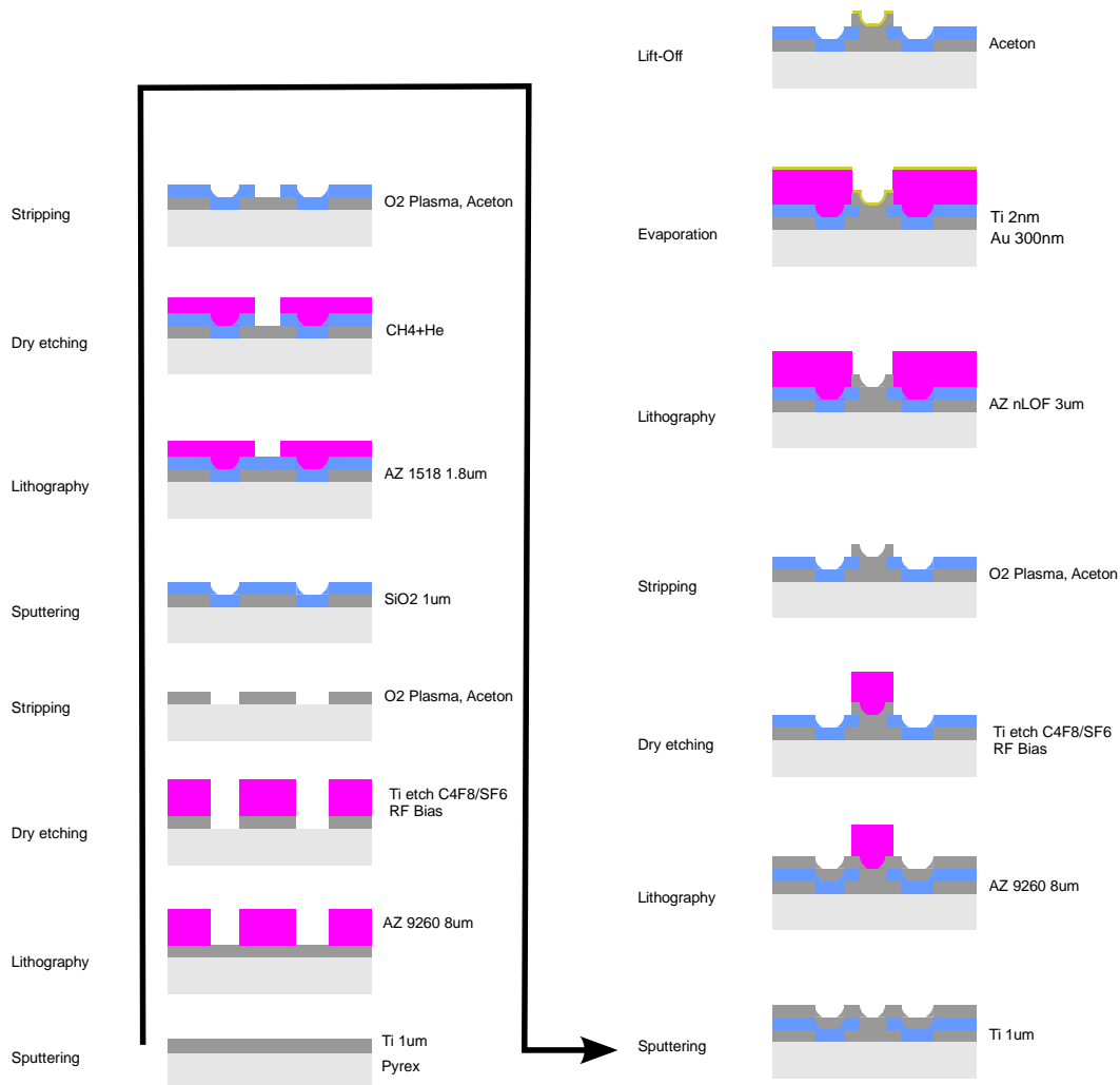
Figure F.4: Fabrication steps (ordered from bottom to top and left to right) for Ziegelstadl v1.1 Wafer #2.
