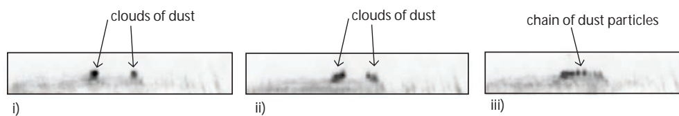
Figure 5.5: Photographs taken of the charged-particle dust trap. The voltage on the addressing RF electrode is lowered (pictures i-iii) and shows how the two point-like traps are morphed into a single linear trap. i) Two point quadrupole ion traps, each with several dust particles. ii) The cloud of particles in each separate trap have enlarged and moved toward each other as the two traps are relaxed. iii) linear trap with a chain of dust particles.
