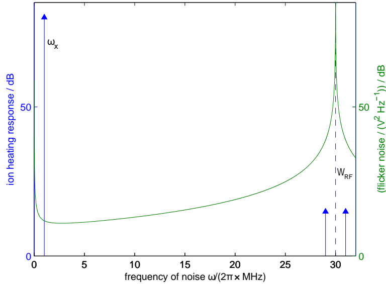
Figure E.4: The relative heating response of the ion overlaid with the expected 1/\Delta f and 1/f voltage noise of a driven thin film conductor (described in text). The 1/\Delta f noise is centered around the carrier frequency \Omega_{\text{rf}} = 2\pi \times 30 MHz. The motional sidebands at \Omega_{\text{rf}} \pm \omega_x can be excited by noise at these frequencies (29 and 31 MHz).
