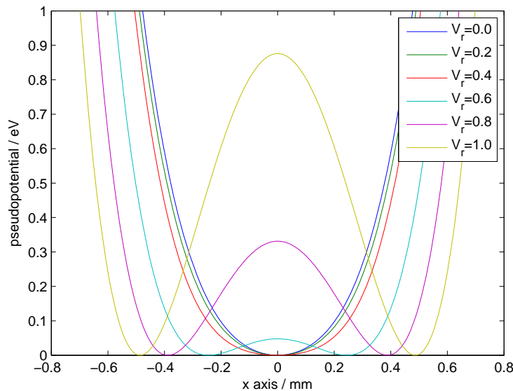
Figure 3.5: The calculated pseudopotential along the x -direction for an electrode structure similar to that shown in figure 3.4, as the voltage ratio V_r = V_{\text{adj}}/V_{\text{nom}} is varied from zero to one. When V_r is zero, there is one well defined trap, as the V_r is increased, two traps appear. When V_r = 1 there are two well defined traps.
