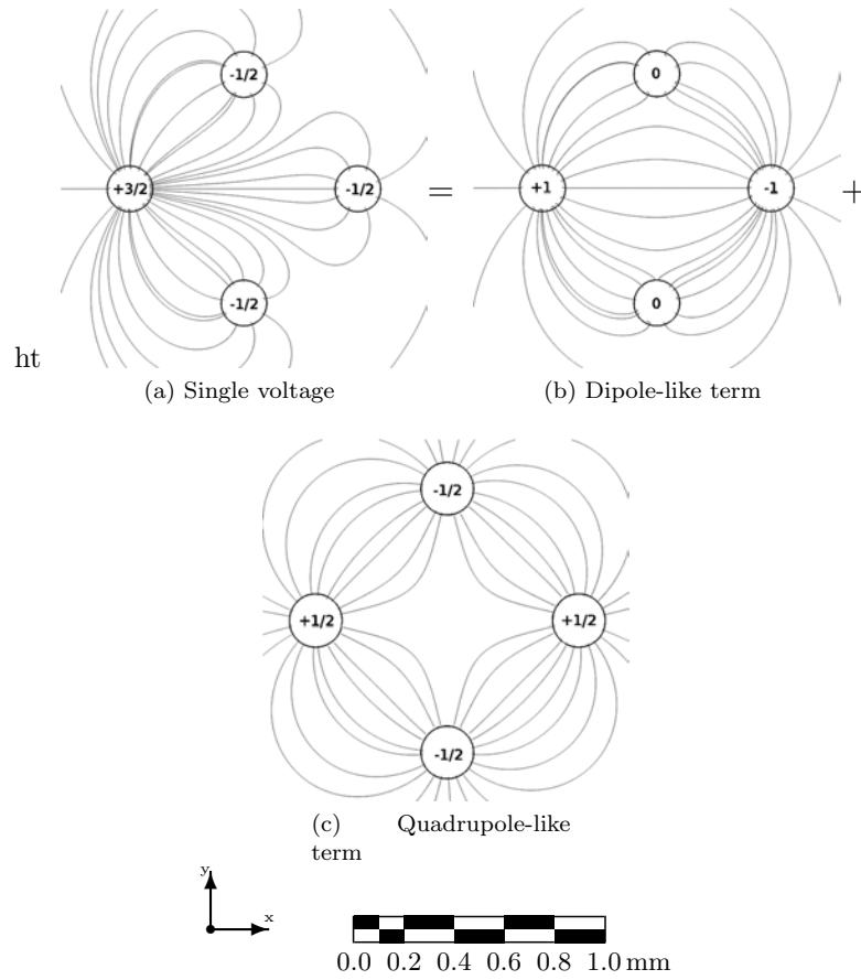
Figure 3.7: Above is the decomposition of the voltage on a single electrode (a) into a dipole-like term (b) and a quadrupole-like term (c).
