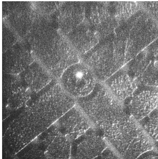
Figure 6.14: A cloud of ^{40}\text{Ca}^+ ions loaded in Folsom over one of the outer trapping sites. The electrode structure (at the focus plane) can be seen below the ions.
