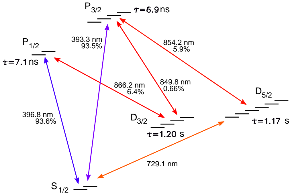
Figure 2.5: Relevant electronic structure of ^{40}\text{Ca}^+ ions. The qubit is typically mapped to the S_{1/2} and D_{5/2} states. Wavelengths of the transitions, lifetimes and branching ratios of the states have been taken from several sources [63–67].
