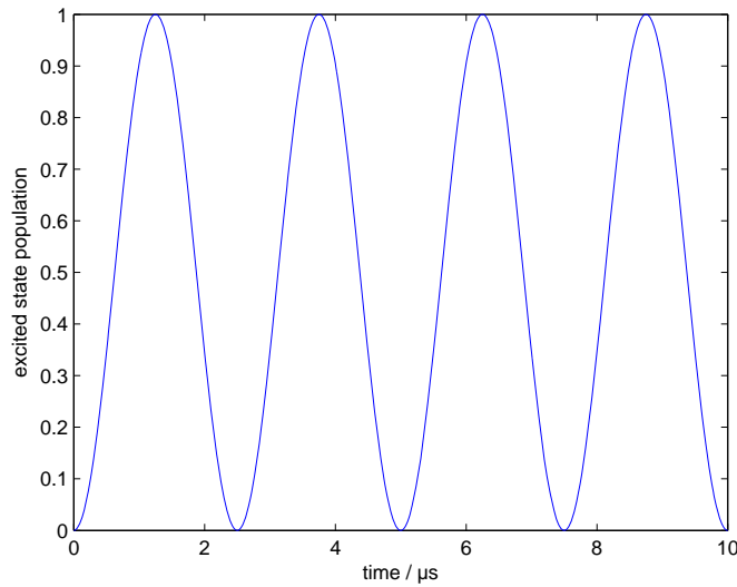
Figure 2.8: Probability of a two level ion being in excited state with applied electromagnetic radiation at the carrier frequency. Shown with an effective Rabi frequency, \Omega_0 , of 2\pi \times 4 \times 10^5 rad/s.
