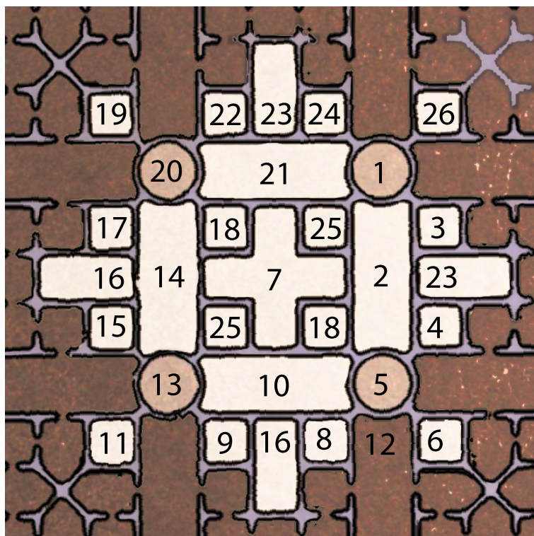
Figure 6.12: Numbering for Folsom’s segmented electrodes is shown above. Some of the electrodes were wired together at the trap, so as to conserve the number of external connections necessary. The internally connected electrodes are shown here with the same number.
