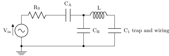
Figure 6.9: Schematic representation of a tank resonator, which uses an impedance matching network of two capacitors C_A and C_B , to match the resonator’s impedance to that of the source impedance R_S of the voltage source V_{in} .
