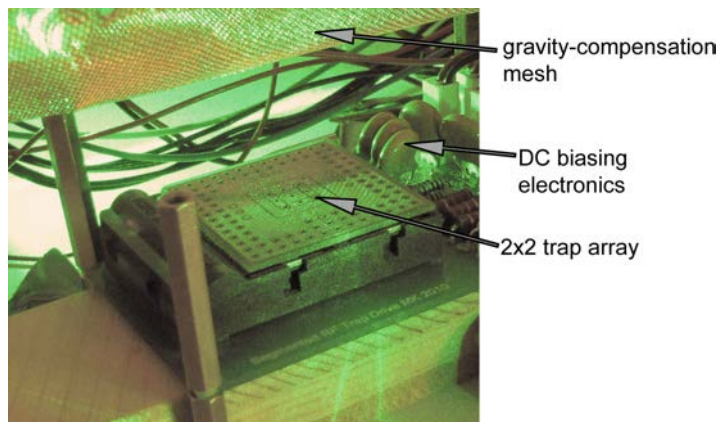
Figure 5.4: Photograph of the test fixture for trapping charged dust particles. The RF electrodes are driven at a voltage of 230 VAC at 50 Hz, with the amplitude tuned via auto-transformers. High-pass filters allow for bias voltages to be applied to all RF electrodes. The entire assembly is housed in an acrylic box to shield it from air currents.
