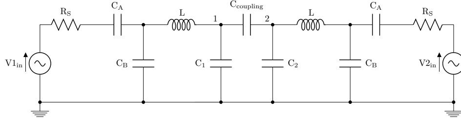
Figure 6.10: Schematic representation of two coupled tank resonators. The capacitor between the two trap electrodes C_{\text{coupling}} is the capacitive coupling caused by the physical proximity of the electrodes on the ion trap. The voltage (amplitude and phase) at node 1 becomes dependent not just on the sinusoidal source V_{1,\text{in}} , but also the voltage at node 2, leading to instabilities in the drive.
