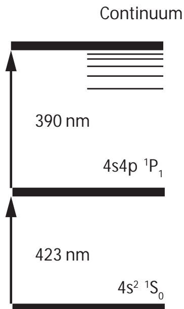
Figure 2.9: The relevant electronic levels for photoionization of neutral calcium (calcium I) to produce singly charged calcium (calcium II). The two-photon process depicted can either directly ionize calcium I or produce Rydberg states. The Rydberg atoms can then be ionized by the electric fields of the ion trap. A resonant laser at the 4s\ ^1S_0 - 4s4p\ ^1P_1 transition allows for the process to be isotope selective. A light source of roughly 390 nm can create Rydberg atoms or a laser with a wavelength shorter than 390 nm could directly ionize the atoms in the 4s4p\ ^1P_1 state.
