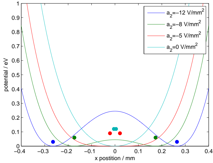
Figure 3.2: The double-well potential \phi as a function of position x for various strengths of the adjustable anti-trapping terms a_2 and a_4 , where the adjustable quartic term scales with a_2 as a_4 = a_2 \times 10^5 \text{ mm}^2 . The fixed terms m_2 and m_4 are kept constant at m_2 = 5 \text{ V/mm}^2 and m_4 = 50 \text{ V/mm}^4 . The quartic term m_4 x^4 , which dominates at large distances, forms an overall trapping potential well. The remaining quadratic terms, which dominate at small distances, can form an anti-trapping potential at the center of the double-well. Circles show the location of trapped ions for various values of a_2 .
