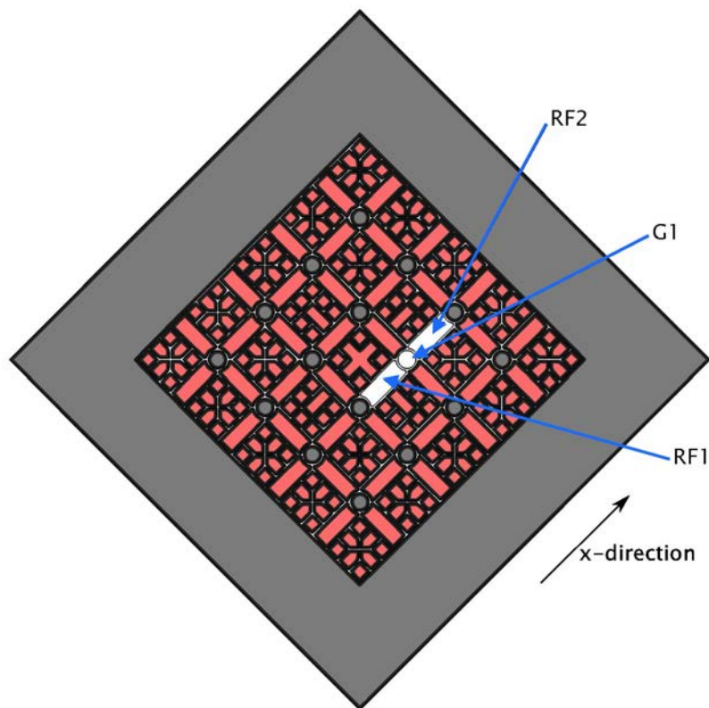
Figure 6.6: Folsom trap RF displacement simulation setup. The electrodes RF1, RF2, and G1 are the relevant electrodes for computing the dipole and quadrupole coefficients around the trapping site electrode G1. The residual RF field from the rest of the RF electrodes (colored red), must also be taken into account.
